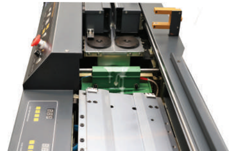
In-line notching, glue application, and nipping station
